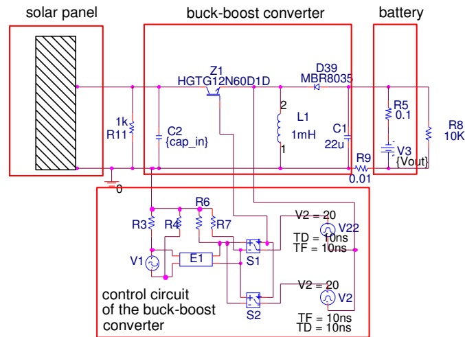
Fig. 5 Control circuit
