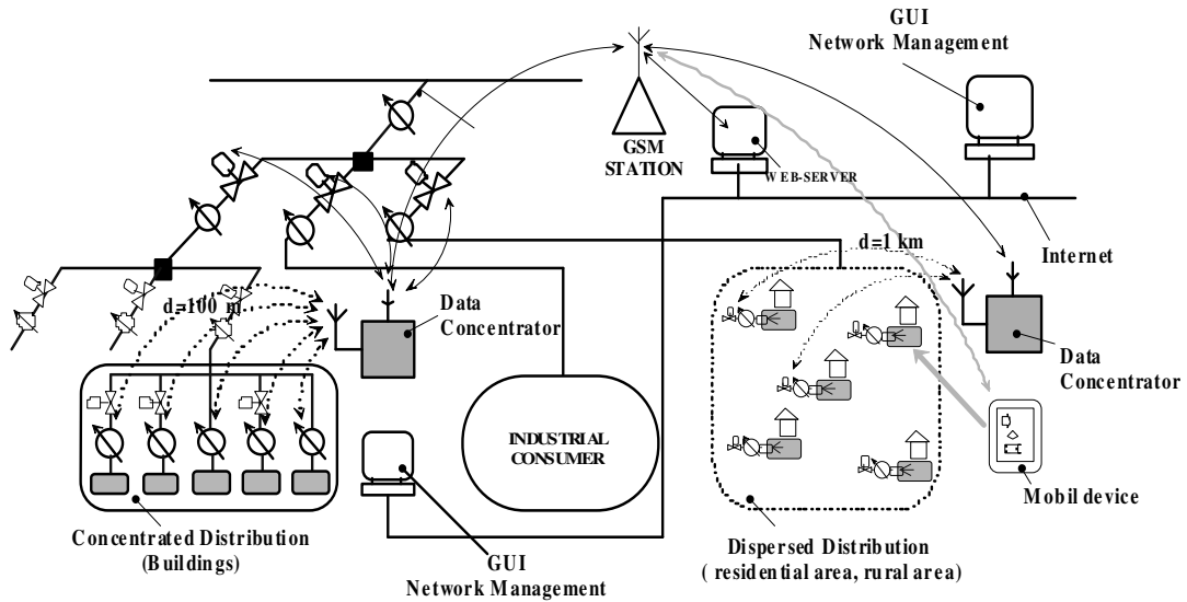
Fig. 6 – Metropolitan network of resource management
