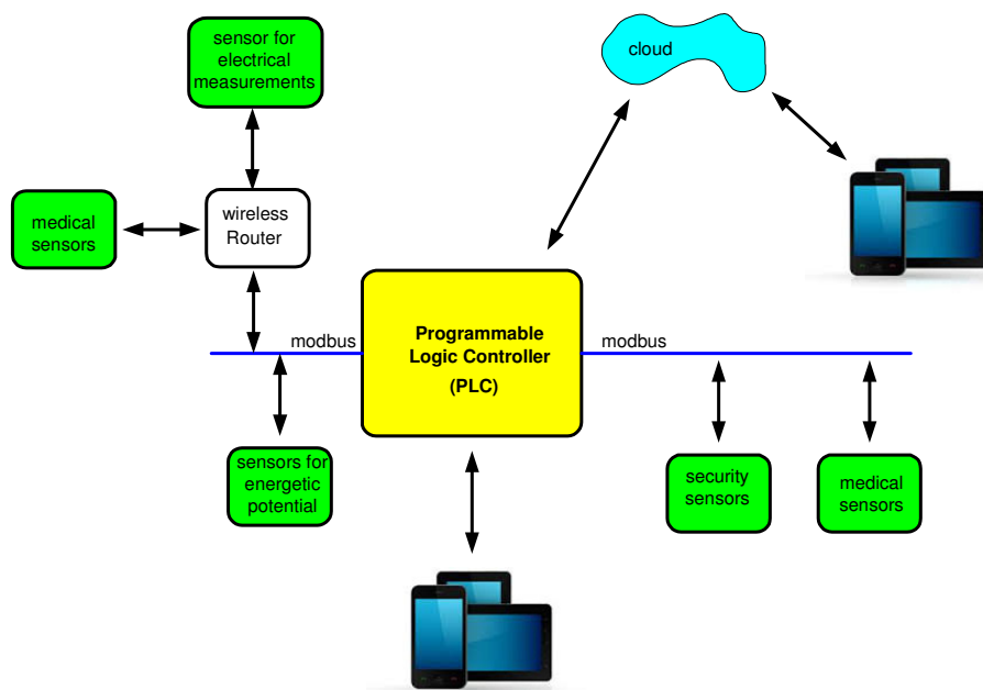
Fig. 1 Block diagram of a reconfigurable system
