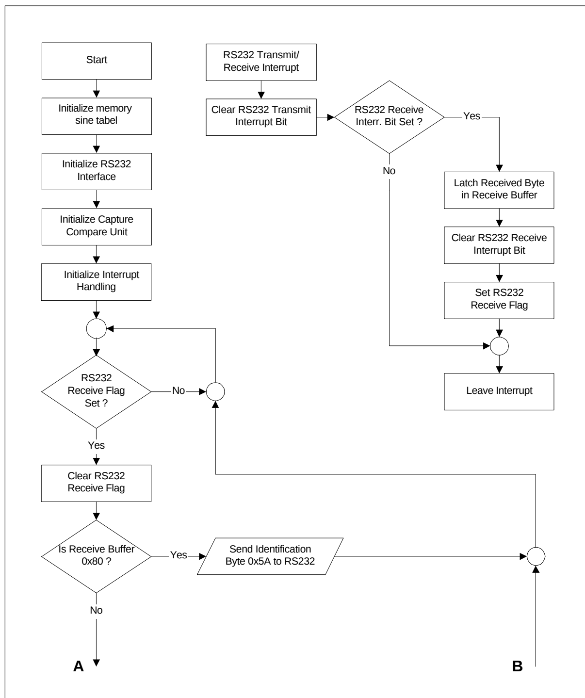
Figure 15: Controller Program Flow-Chart and RS 232 Interrupt Service Routine
