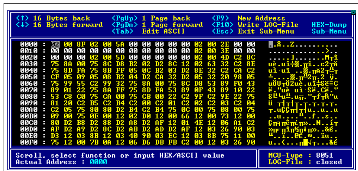
Figure 8 : Hex-Dump Function of ADIS51
