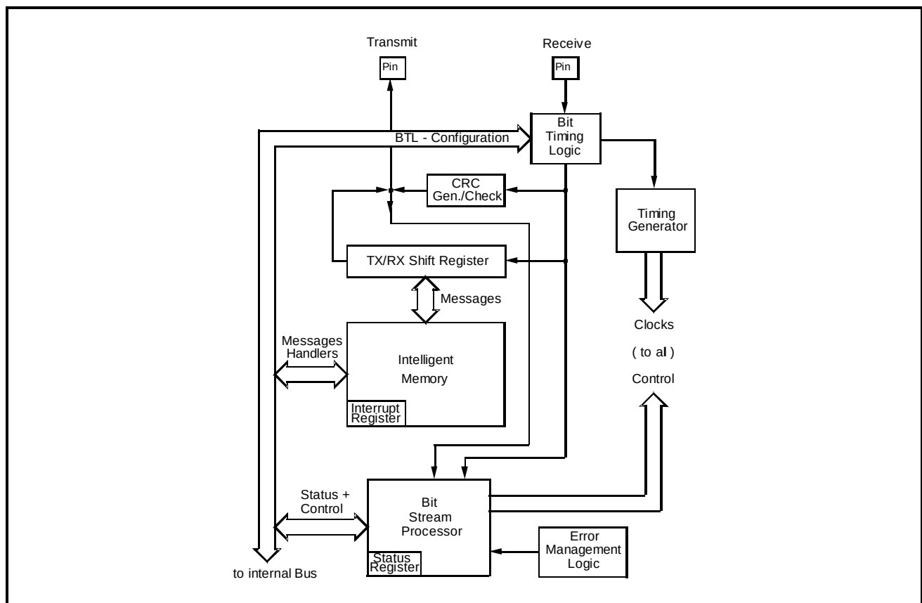
Figure 3.2-2: Block Diagram of the CAN Controller on the C167CR / C515C
