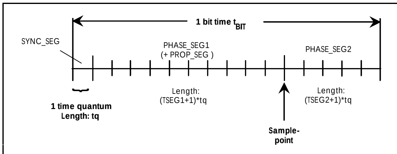
Figure 5.3-1: Rough Structure of one Bit Cell in the CAN Module of the C167CR / C515C and in the SAE 81C90/91
