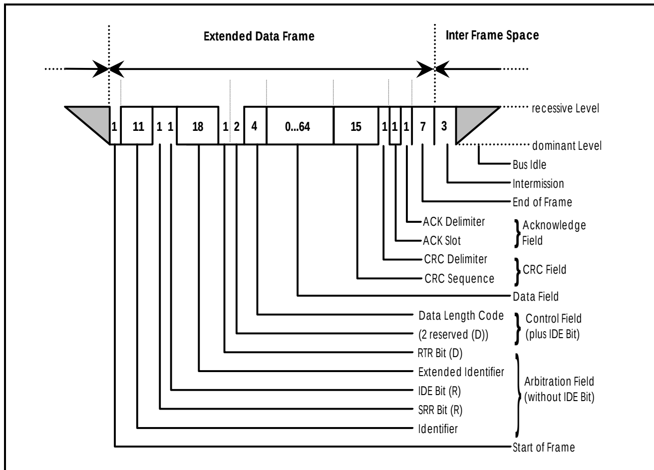
Figure 2.3-2: Extended CAN Data Frame
