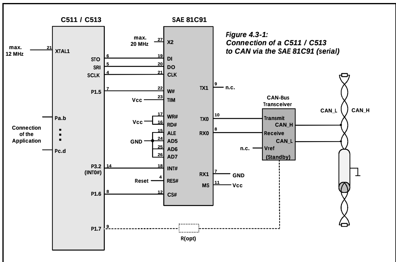
Figure 4.3-1: Connection of a C511 / C513 to CAN via the SAE 81C91 (serial)
