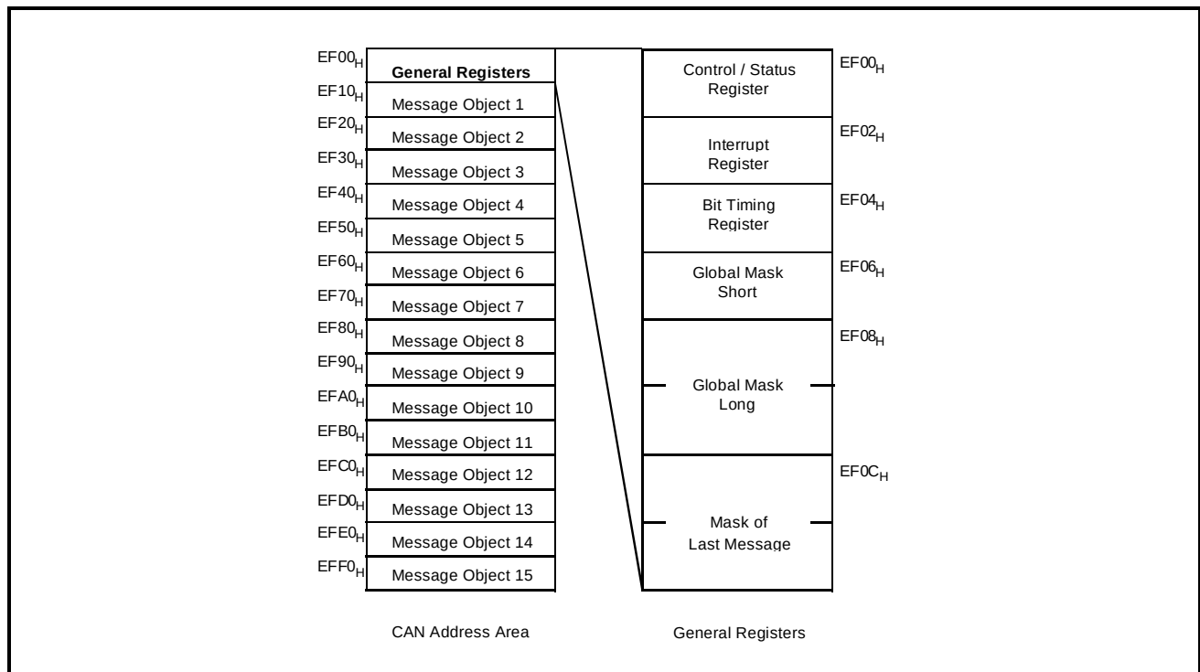
Figure 3.2-3b: CAN addressing area on the C167CR
