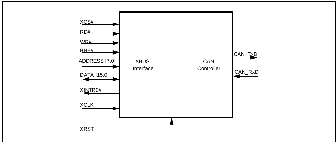
Figure 3.2-1: Block Diagram of the CAN module (connected to the C167CR here)
