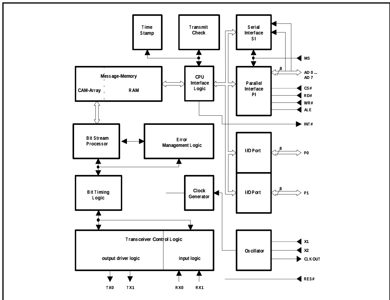
Figure 3.3-1: Block Diagram of the SAE 81C90/91 (I/O Ports only available for SAE 81C90)
