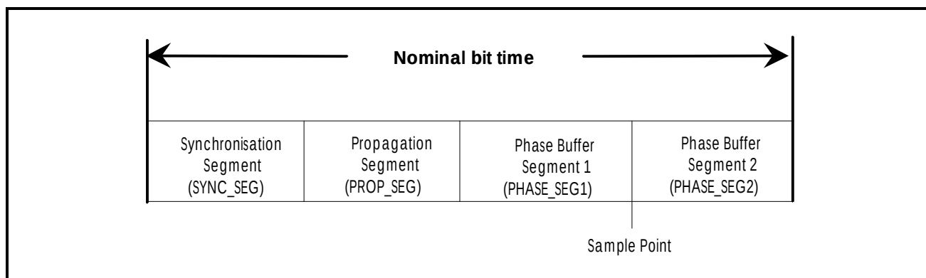
Figure 2.4-1: Partition of bit time
