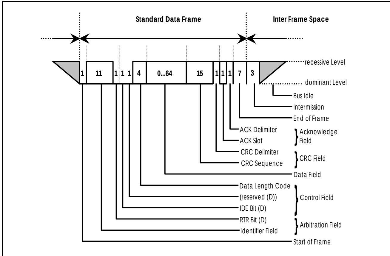
Figure 2.3-1: Standard CAN Data Frame
