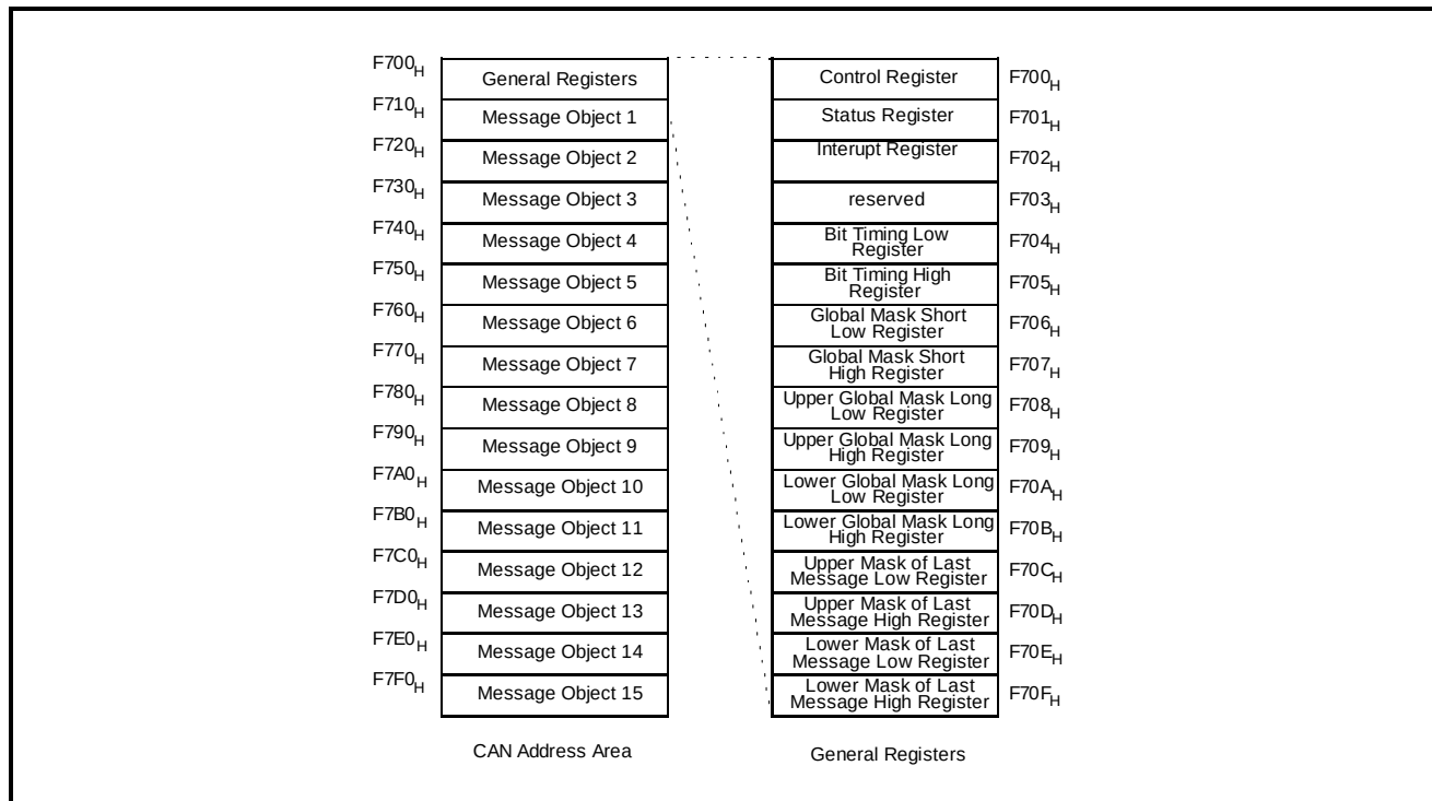
Figure 3.2-3a: CAN addressing area on the C515C
