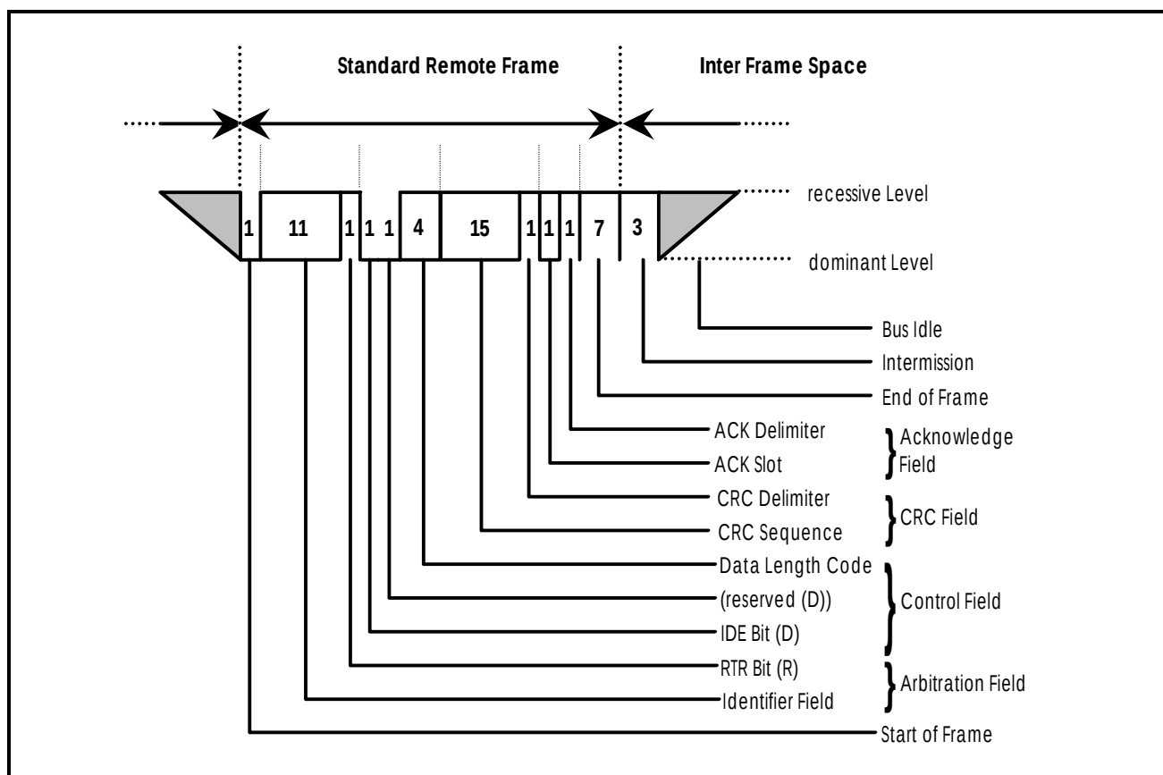
Figure 2.3-3: Standard CAN Remote Frame
