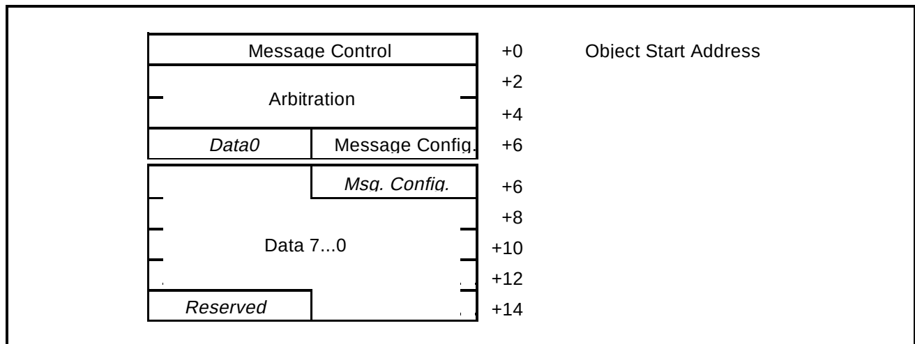
Figure 3.2-4b: Message Objects in the C167CR
