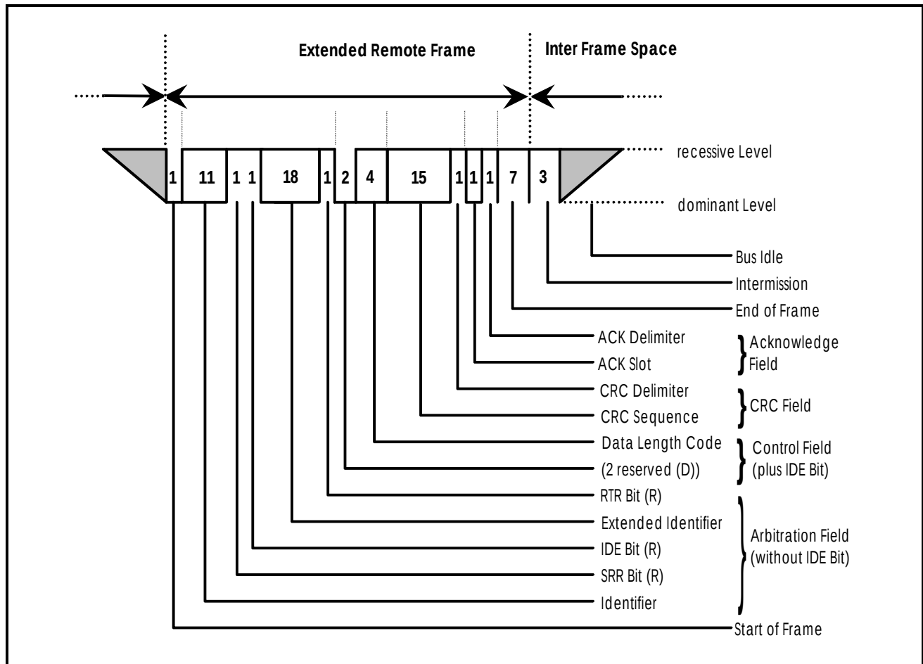
Figure 2.3-4: Extended CAN Remote Frame
