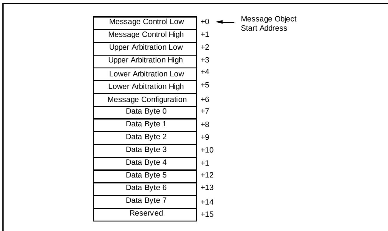
Figure 3.2-4a: Message Objects in the C515C
